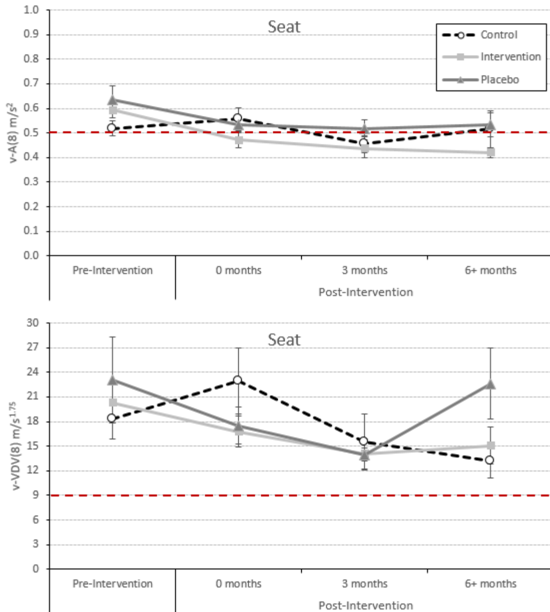
Figure 6. Comparison of the vector sum daily average weighted vibration ( vA(8) ) and daily vibration base values ( vVDV(8) ) between the seats over time. The red dotted line stands for the ISO action limits 0.5 m/s^2 for A(8) and 9.1 m/s^{1.75} for VDV(8) .
