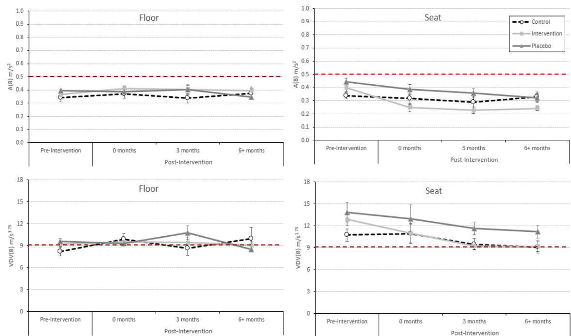
Figure 3. Comparison of the daily average weighted vibration ( A(8) ) and daily Vibration Dose Values ( VDV(8) ) between the three study groups over time. The red dotted lines represent the ISO and EU action limits, 0.5 \text{ m/s}^2 for A(8) and 9.1 \text{ m/s}^{1.75} for VDV(8) , for exposure to WBV. Note that pre-intervention WBV measurements are based on the original air suspension seats and not from the seats installed or used after the intervention. Due to the substantial number of study dropouts, subject turnover and new trucks, 12 month values are not presented.
