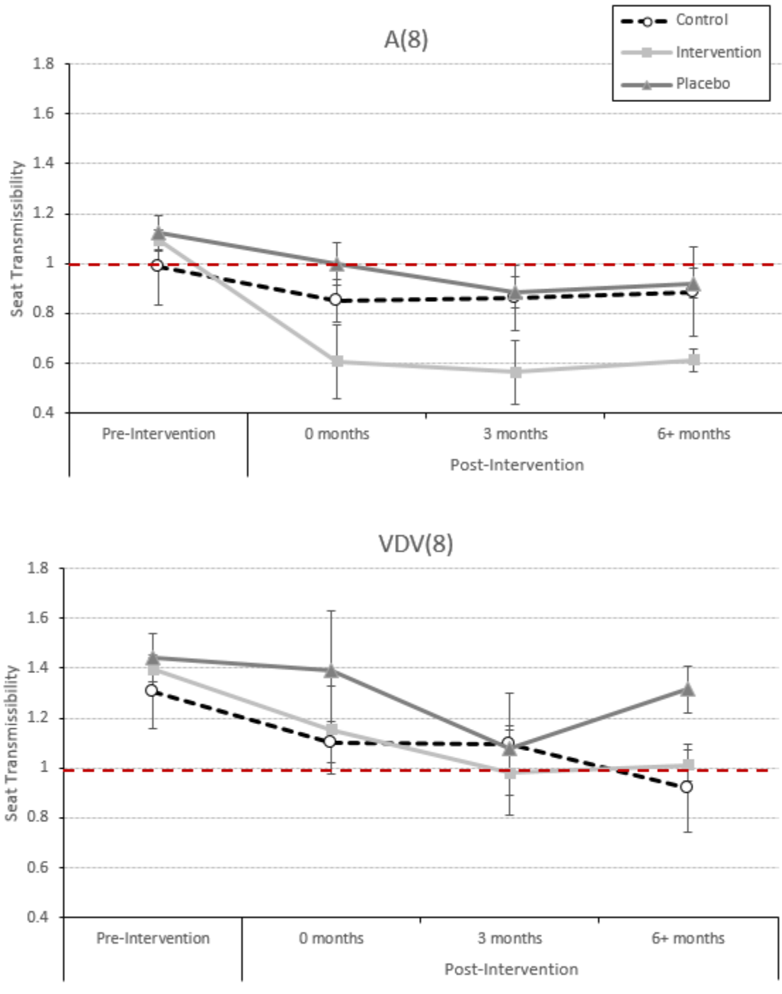
Figure 4. Comparison of Seat Transmissibility (%) between the groups based on the daily average weighted vibration (A(8)) and daily vibration dose value (VDV(8)). Values above the red dotted line indicates that the seat is amplifying rather than attenuating the floor-transmitted vibration.
